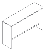
PSW58 1800 / 500 / 1100 52.25 kg
