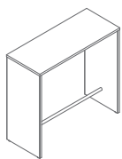
PSW52 1200 / 500 / 1100 42.3 kg
