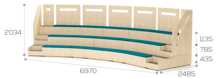
26 seat configuration
