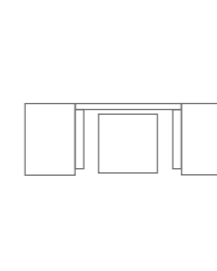
Two Seat Diner Units Footprint: W2020 x D780 (min)
